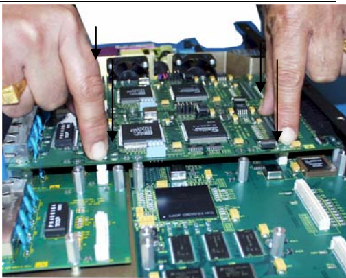
Figure 3.6.2f: Securely latching up 6KPM Cards into a Magnum 6K16V
